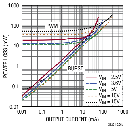
Power Loss, V_{OUT} = 6.9\text{V}
