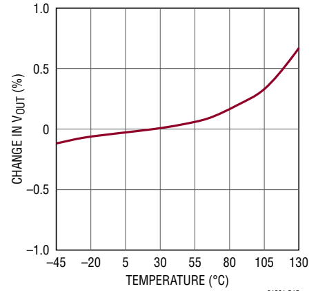
Output Voltage vs Temperature (Normalized to 25^\circ\text{C} )
