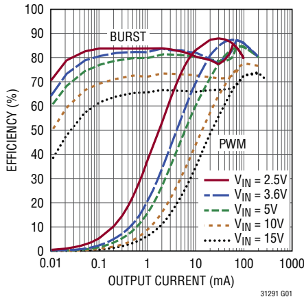
Efficiency, V_{OUT} = 2.5\text{V}
