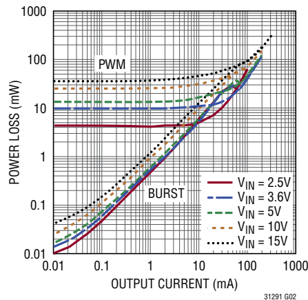
Power Loss, V_{OUT} = 2.5\text{V}
