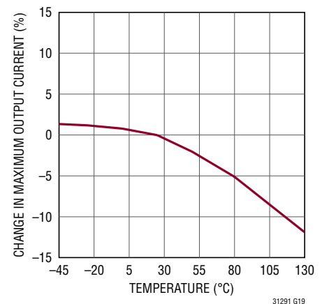
Maximum Output vs Temperature (Normalized to 25^\circ\text{C} )
