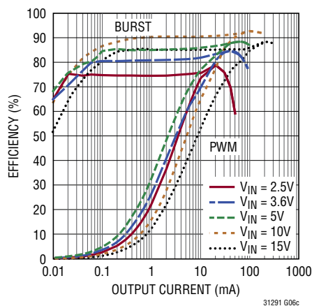
Efficiency, V_{OUT} = 8.2\text{V}
