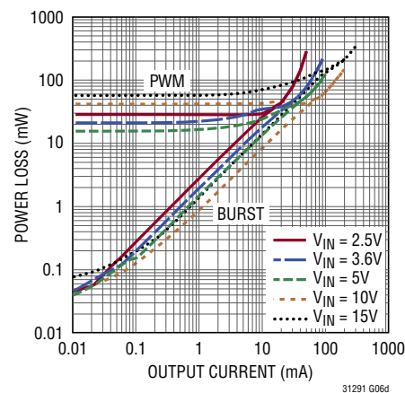
Power Loss, V_{OUT} = 8.2\text{V}
