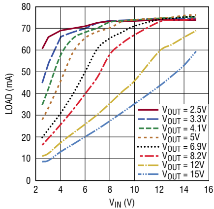
Burst Mode Threshold vs V_{IN} and V_{OUT}
