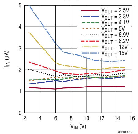
No Load Input Current vs V_{IN} and V_{OUT} (PWM = 0V)
