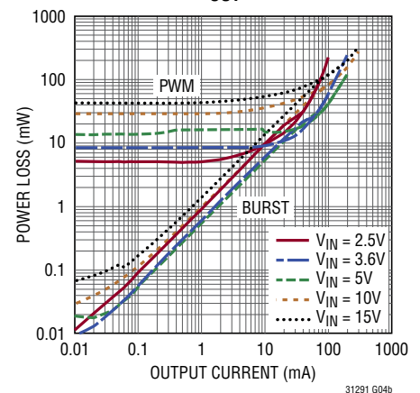
Power Loss, V_{OUT} = 4.1\text{V}
