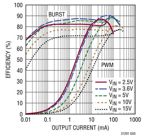
Efficiency, V_{OUT} = 3.3\text{V}
