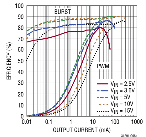
Efficiency, V_{OUT} = 6.9\text{V}
