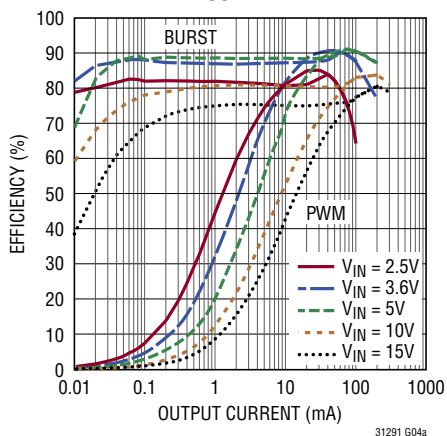
Efficiency, V_{OUT} = 4.1\text{V}
