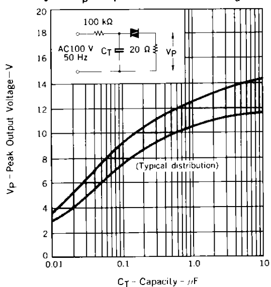
Fig. 5 V_p - C_T CHARACTERISTIC ( T_a = 25^\circ\text{C} )
