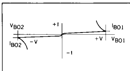
Fig. 1 FUNDAMENTAL CHARACTERISTIC
