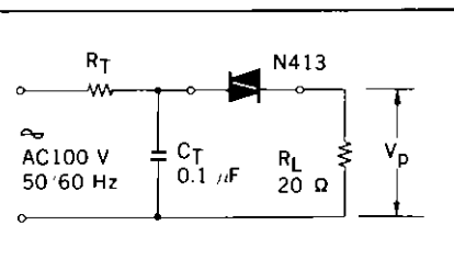
Fig. 2 FUNDAMENTAL CIRCUIT
