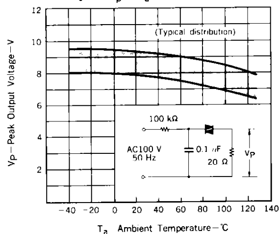
Fig. 4 V_p - T_a CHARACTERISTIC
