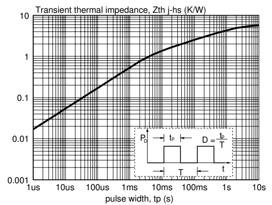
Fig.11. Transient thermal impedance; Z_{th\ j-hs} = f(t_p) .
