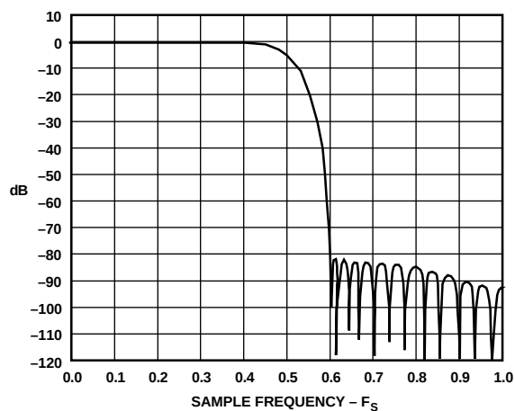
Figure 26. AD1847 Digital-to-Analog Frequency Response (Full-Scale Inputs, 0 dB Attenuation)
