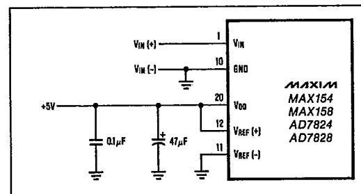
Figure 8c. Power Supply as Reference
