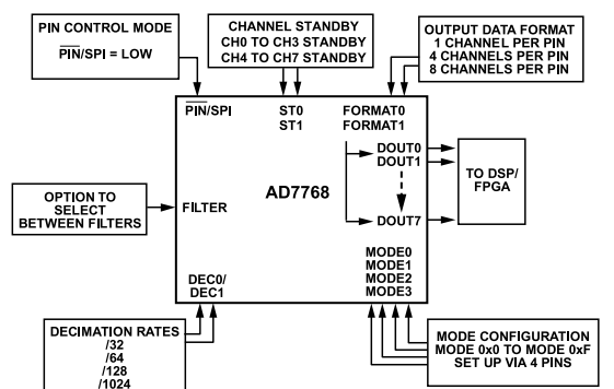
Figure 76. AD7768 Pin Configurable Functions
