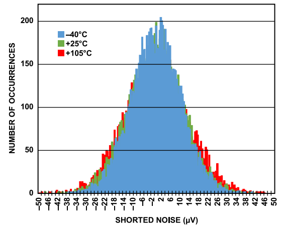
Figure 28. Shorted Noise at Different Temperatures, Wideband Filter
