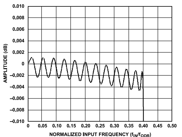
Figure 91. Wideband Filter Pass-Band Ripple
