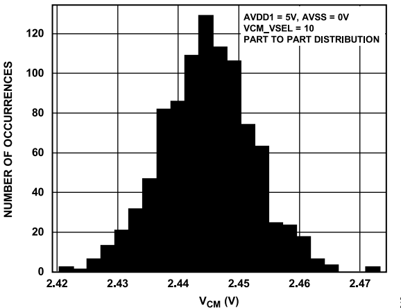
Figure 64. VCM Output Voltage Distribution
