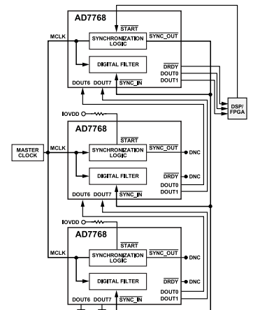
Figure 109. Daisy-Chaining Multiple AD7768 Devices
