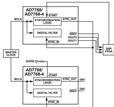
Figure 110. Synchronizing Multiple AD7768/AD7768-4 Devices Using SYNC OUT
