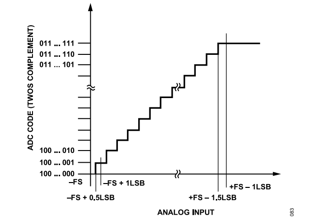
Figure 82. ADC Ideal Transfer Functions (FS is Full Scale)
