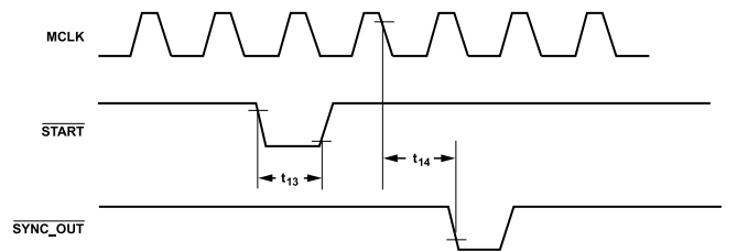
Figure 5. Asynchronous START and SYNC_OUT Timing Diagram
