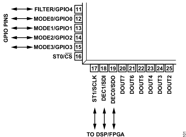
Figure 113. AD7768 GPIO Functionality
