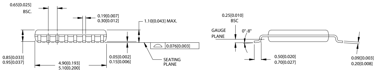
Figure 6. 16-Pin (150-Mil) QSOP Q1
