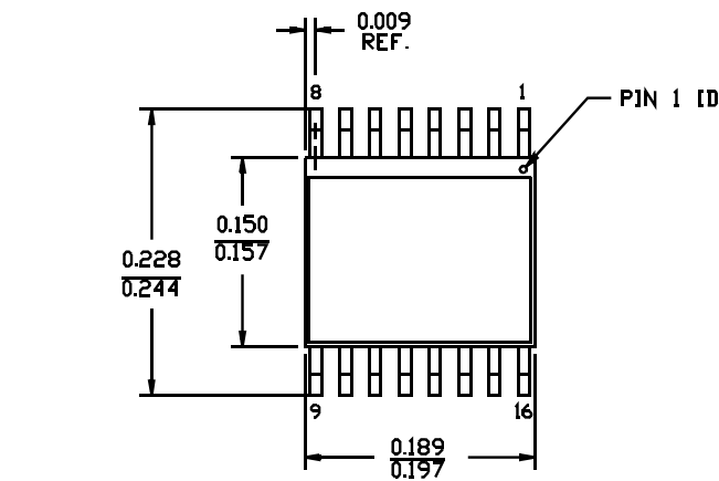
Figure 6. 16-Pin (150-Mil) QSOP Q1
