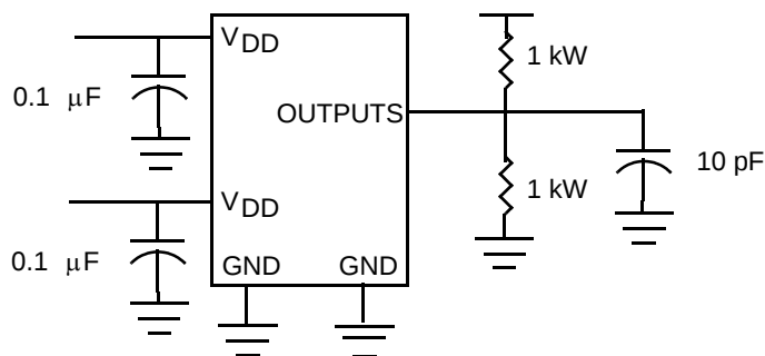
Test Circuit # 2
