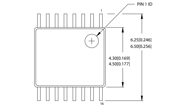
Figure 5. 16-Pin TSSOP 4.40 mm Body Z16.173
