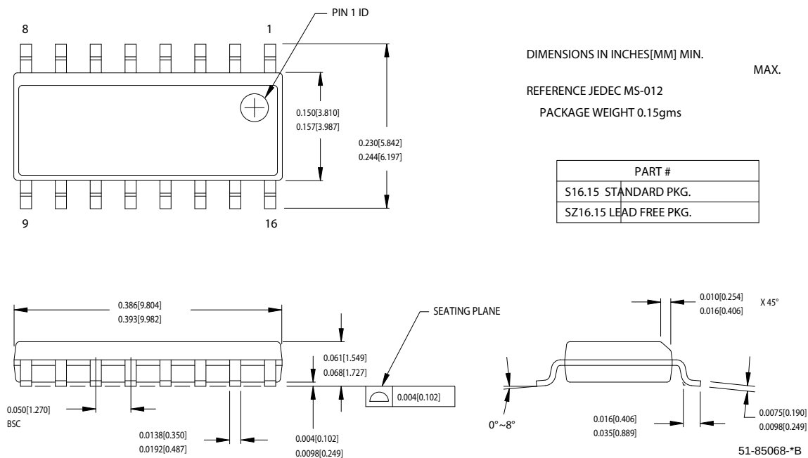
Figure 4. 16-Pin (150-Mil) SOIC S16.15
