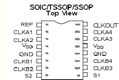
Figure 1. Pin Diagram - CY23S09
