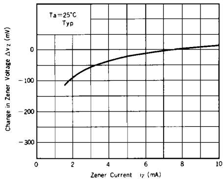
Fig. 5 \Delta V_z - I_z Characteristic
