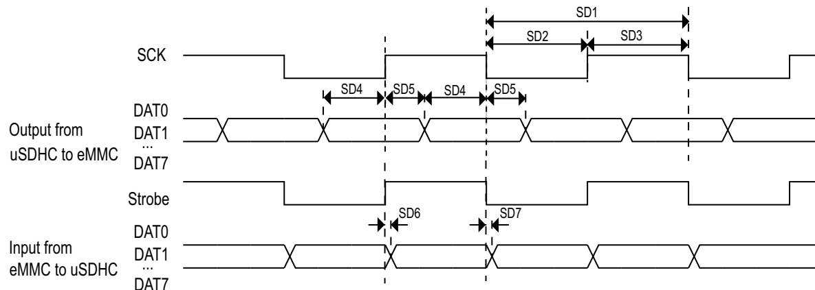
Figure 43. HS400 timing
