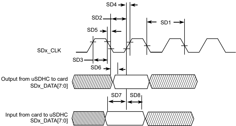
Figure 39. SD/eMMC4.3 timing
