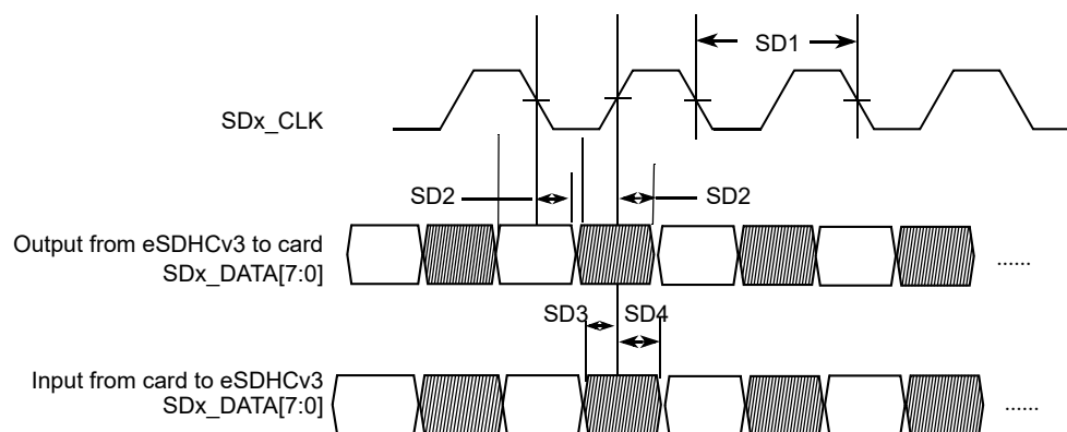
Figure 40. eMMC4.4/4.41/SD3.0 timing
