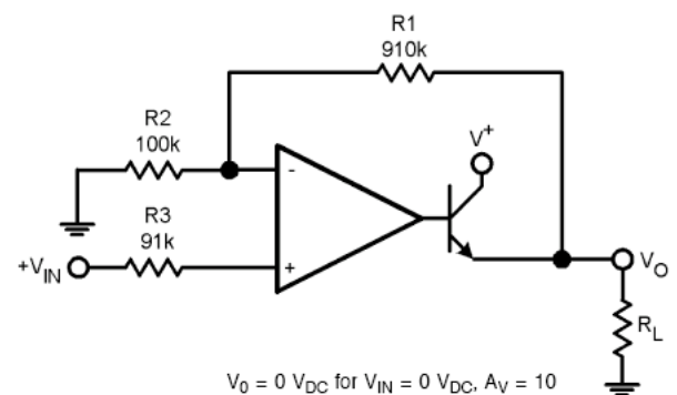
Figure 6. Power Amplifier
