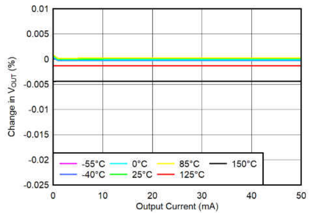
Figure 6-25. Load Regulation at Light Load
