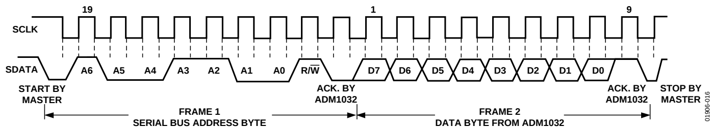
Figure 16. Reading Data from a Previously Selected Register
