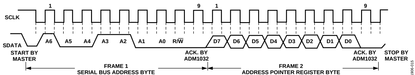
Figure 15. Writing to the Address Pointer Register Only
