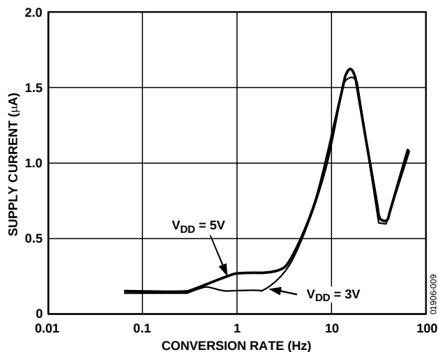
Figure 9. Operating Supply Current vs. Conversion Rate
