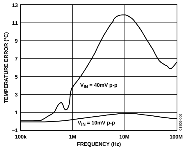
Figure 6. Temperature Error vs. Differential Mode Noise Frequency
