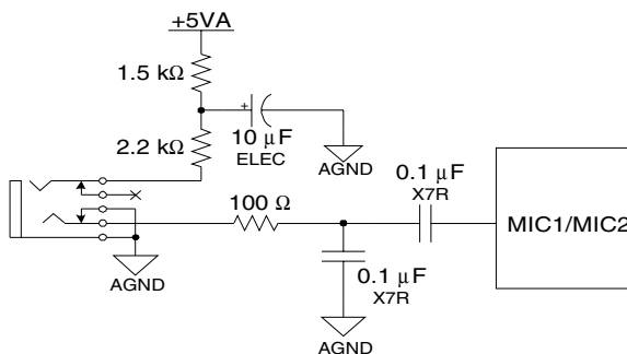
Figure 28. Microphone Input
