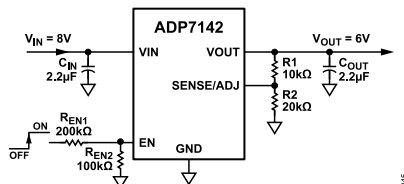
Figure 47. Typical EN Pin Voltage Divider
