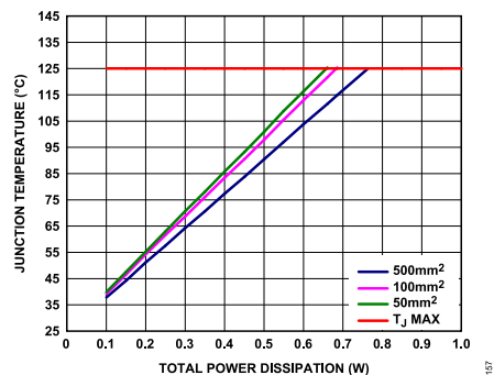
Figure 58. TSOT, T_A = 25^\circ\text{C}
