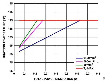
Figure 57. SOIC, T_A = 85^\circ\text{C}
