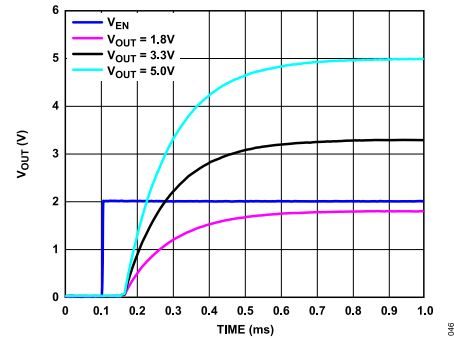
Figure 48. Typical Start-Up Behavior
