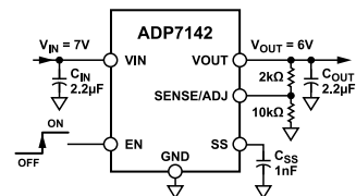
Figure 2. ADP7142 with 5 V Output Adjusted to 6 V
