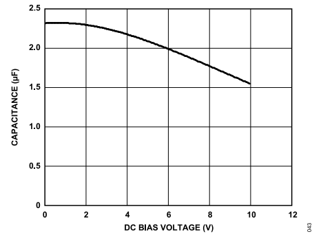
Figure 45. Capacitance vs. Voltage Characteristic
