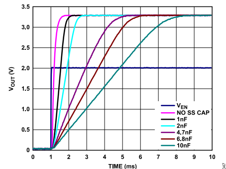
Figure 49. Typical Soft Start Behavior, Different C_{SS}
