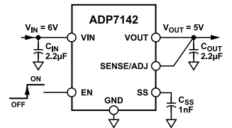
Figure 1. ADP7142 with Fixed Output Voltage, 5 V
