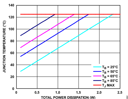
Figure 63. TSOT Junction Temperature Rise, Different Board Temperatures
