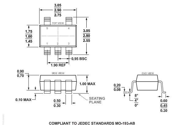
Figure 69. 5-Lead Thin Small Outline Transistor Package [TSOT] (UJ-5)
