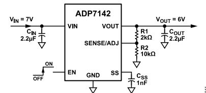
Figure 43. Typical Adjustable Output Voltage Application Schematic
