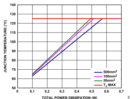
Figure 59. TSOT, T_A = 50^\circ\text{C}
