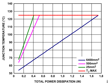
Figure 54. LFCSP, T_A = 85^\circ\text{C}
