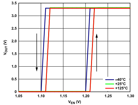
Figure 46. Typical VOUT Response to EN Pin Operation
