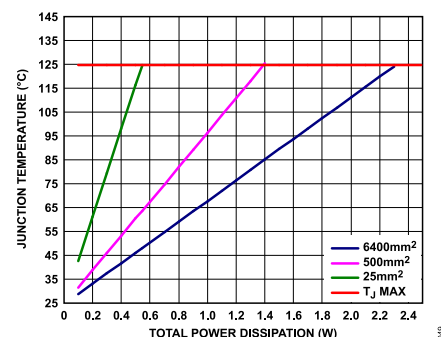
Figure 52. LFCSP, T_A = 25^\circ\text{C}
