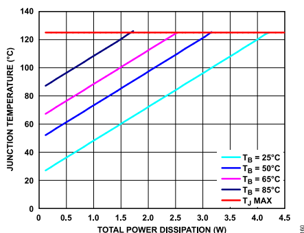
Figure 61. LFCSP Junction Temperature Rise, Different Board Temperatures
