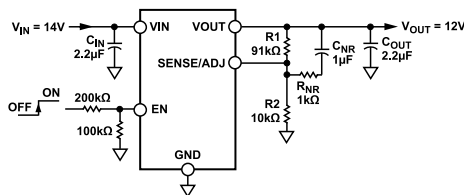
Figure 50. Noise Reduction Modification
