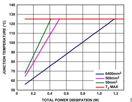
Figure 56. SOIC, T_A = 50^\circ\text{C}
