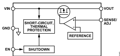
Figure 42. Internal Block Diagram
