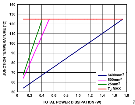
Figure 53. LFCSP, T_A = 50^\circ\text{C}
