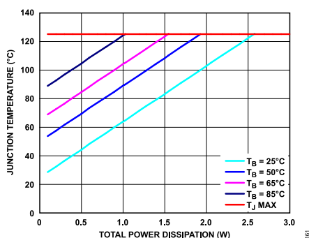
Figure 62. SOIC Junction Temperature Rise, Different Board Temperatures
