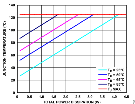
Figure 55. SOIC, T_A = 25^\circ\text{C}
