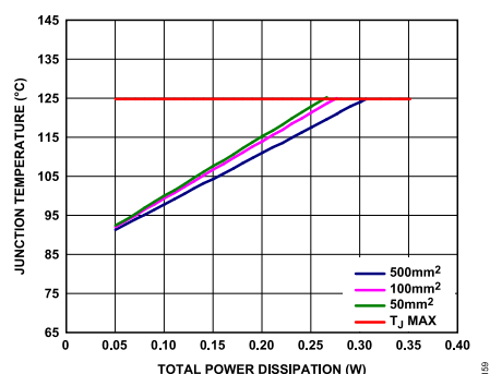
Figure 60. TSOT, T_A = 85^\circ\text{C}
