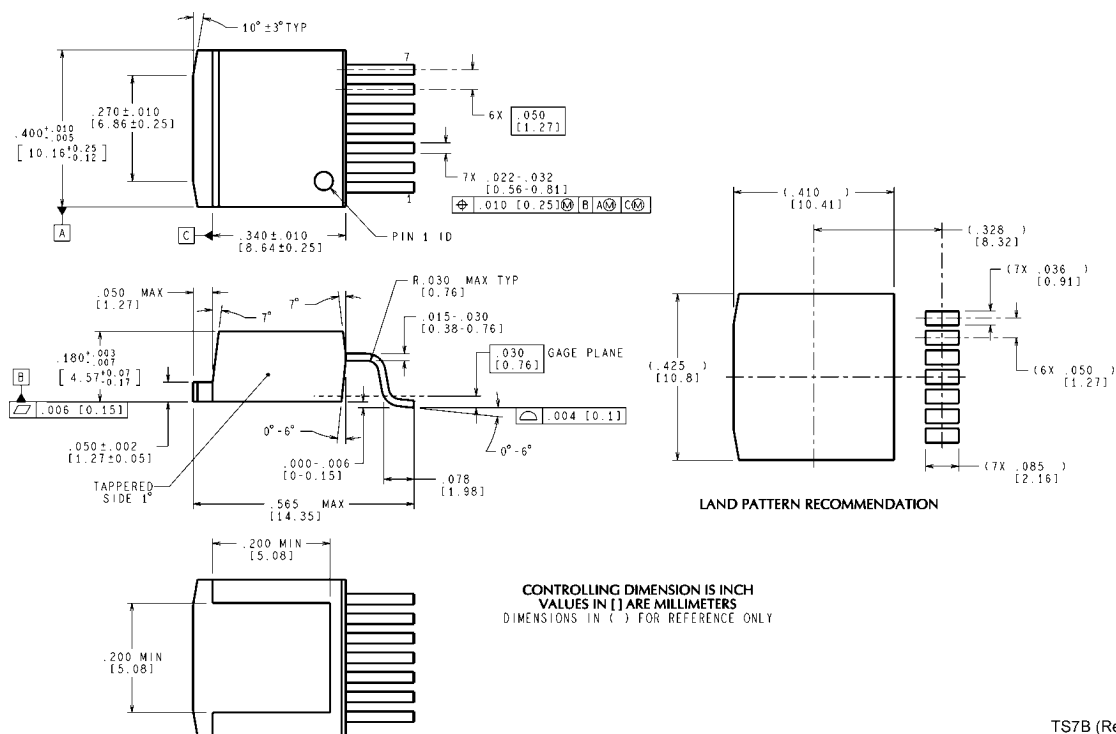
TO-263 7-Lead, Molded, Surface Mount Package (TO263-7) NS Package Number TS7B
