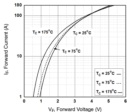
Figure 17. Forward Characteristics
