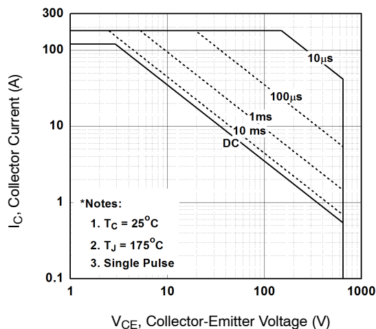
Figure 16. SOA Characteristics
