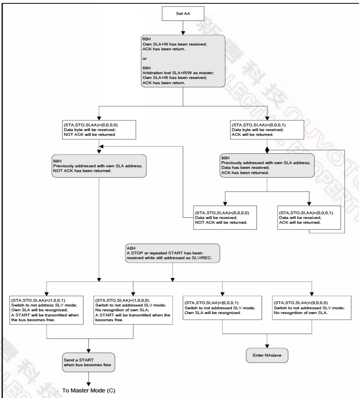
Figure 18-8 Slave Receiver Mode
