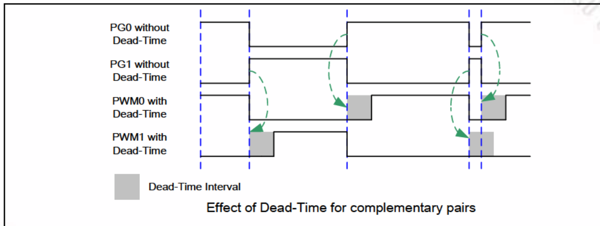
Figure 25-13: Dead-Time Insertion
