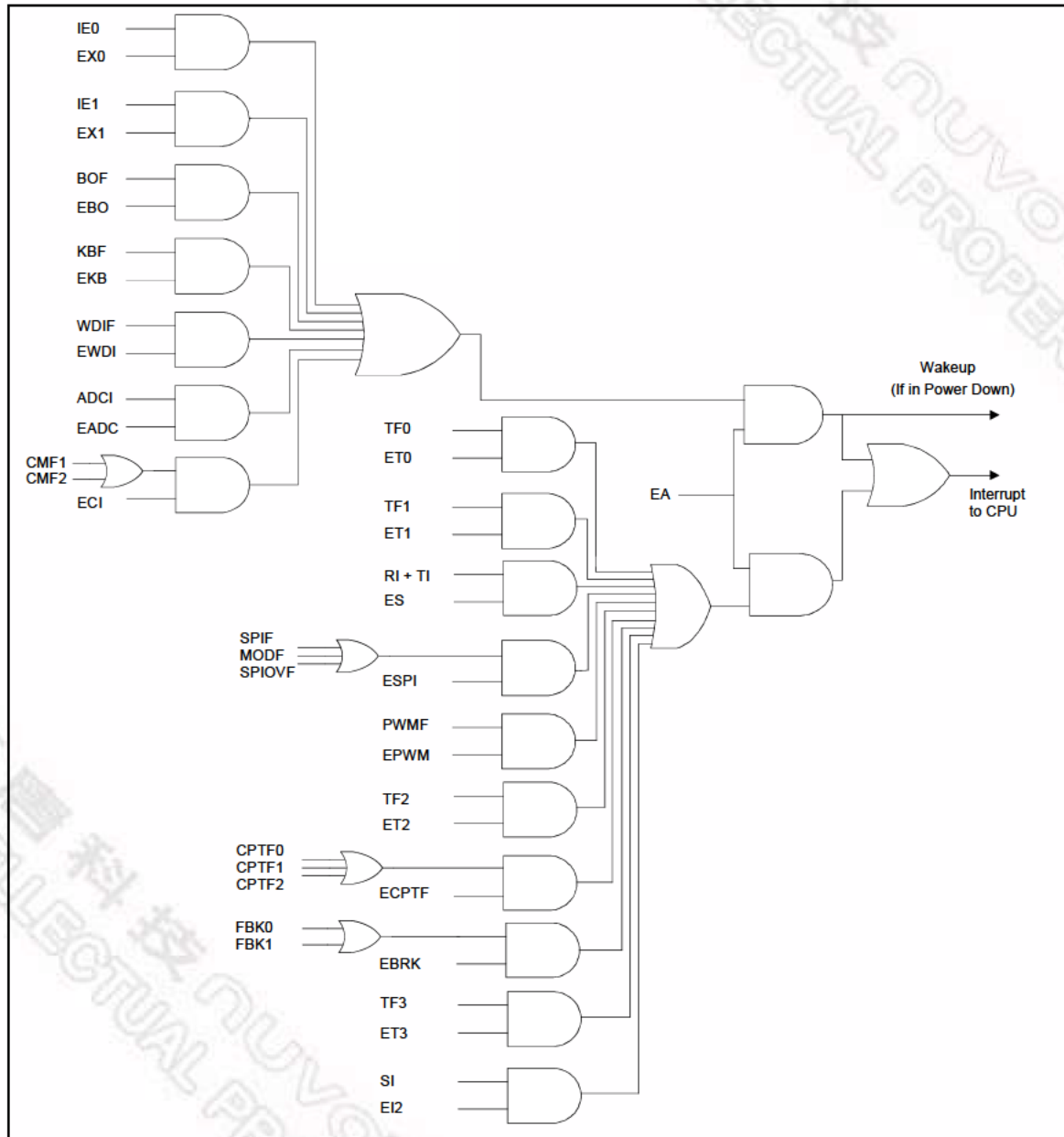
Figure 11-1 Interrupt Source
