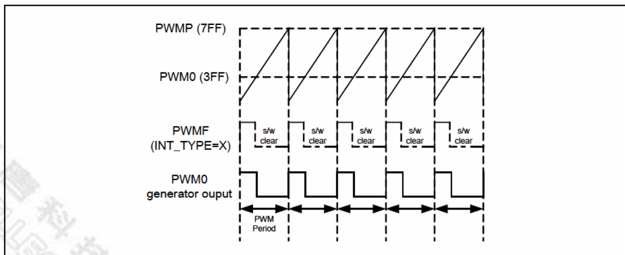
Figure 25-4: PWM0 Edge Aligned Waveform Output
