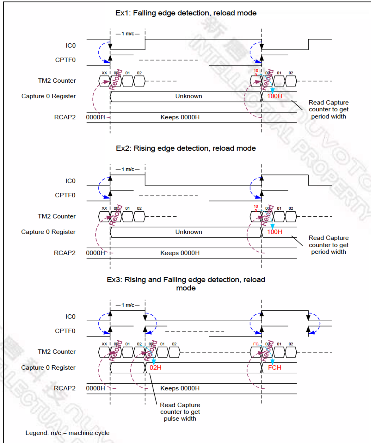
Figure 15-3 Timing diagram for Input Capture, IC0
