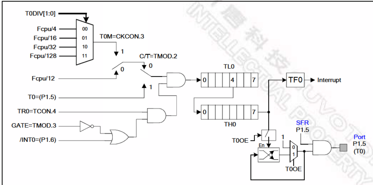
Figure 13-1 Timer 0 Mode 0
