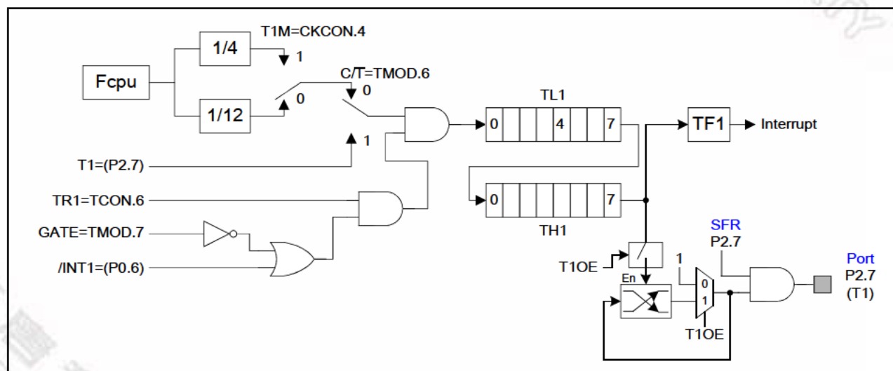
Figure 13-4 Timer 1 Mode 1
