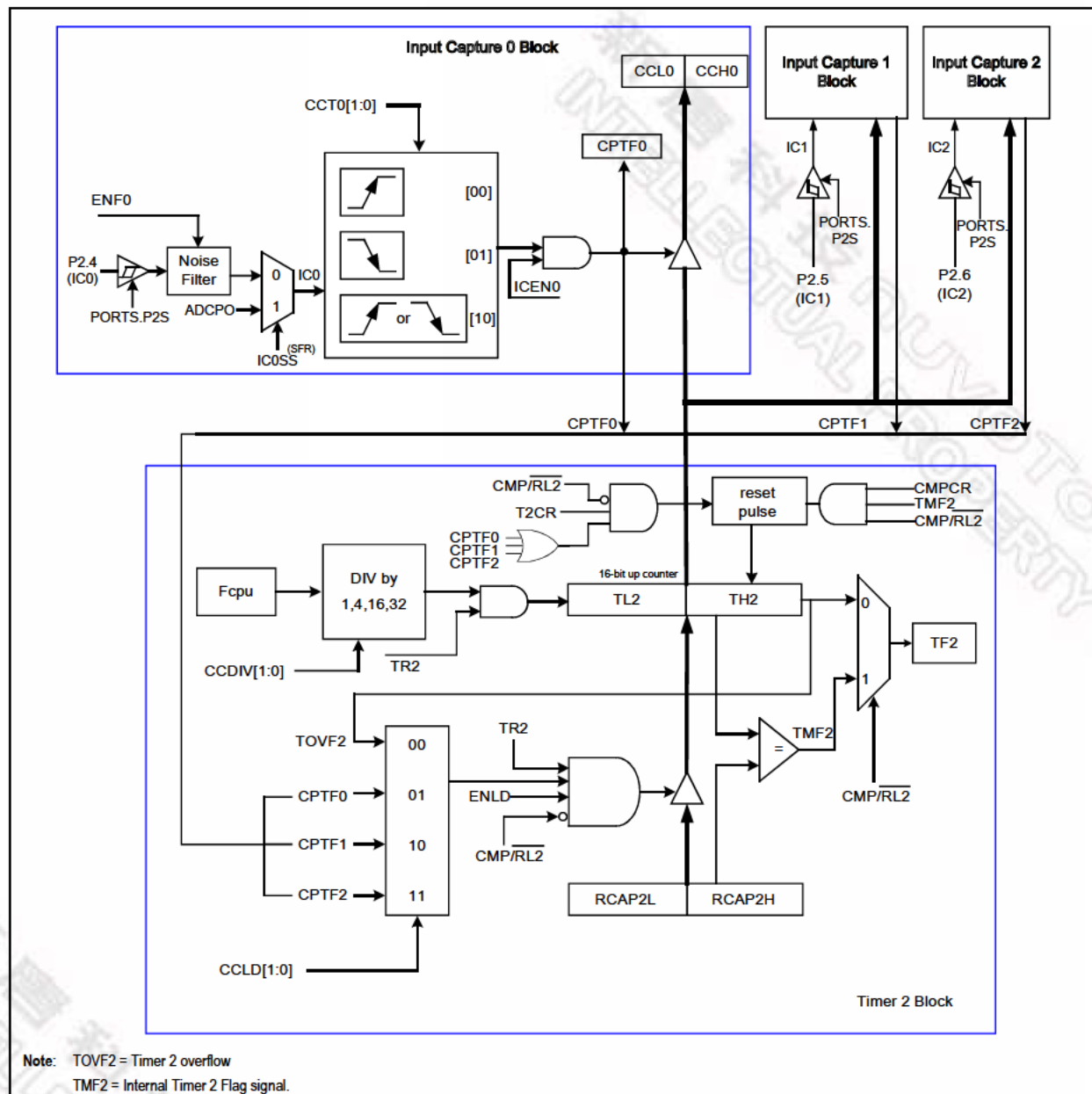
Figure 15-2 Timer2/capture modules
