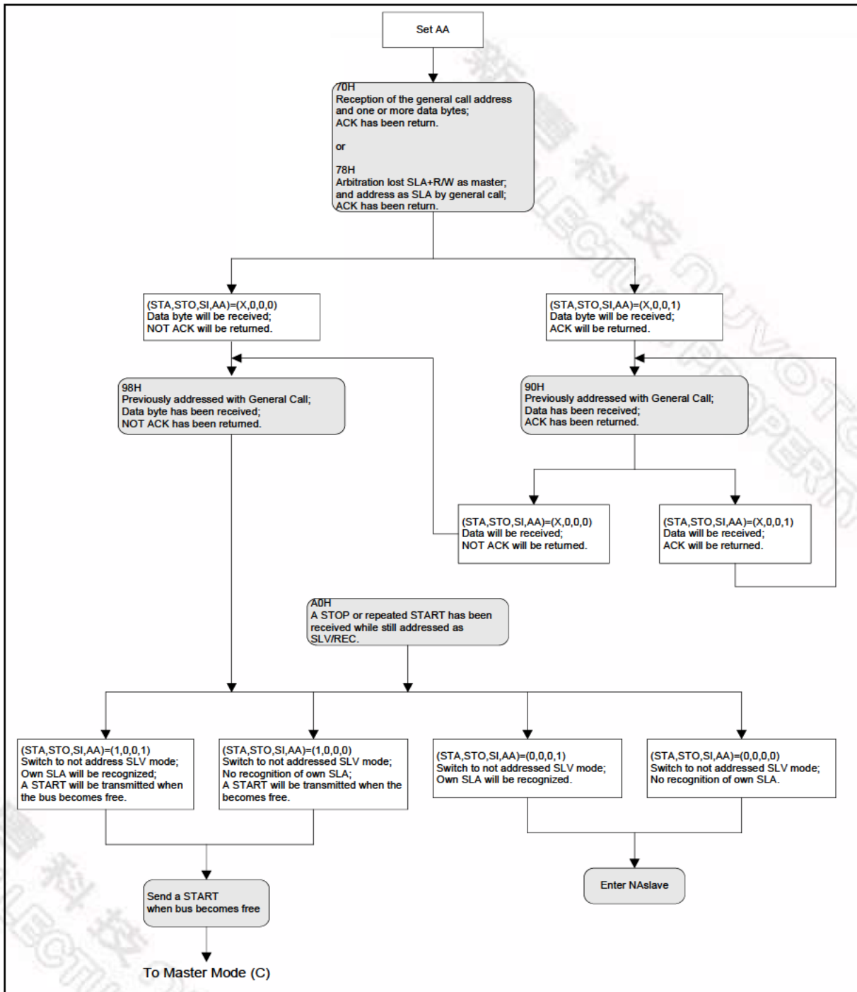
Figure 18-9 GC Mode
