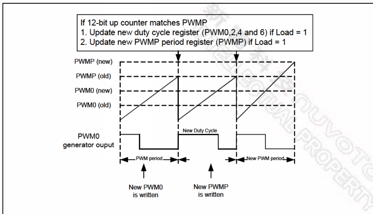
Figure 25-3: Edge-Aligned PWM
