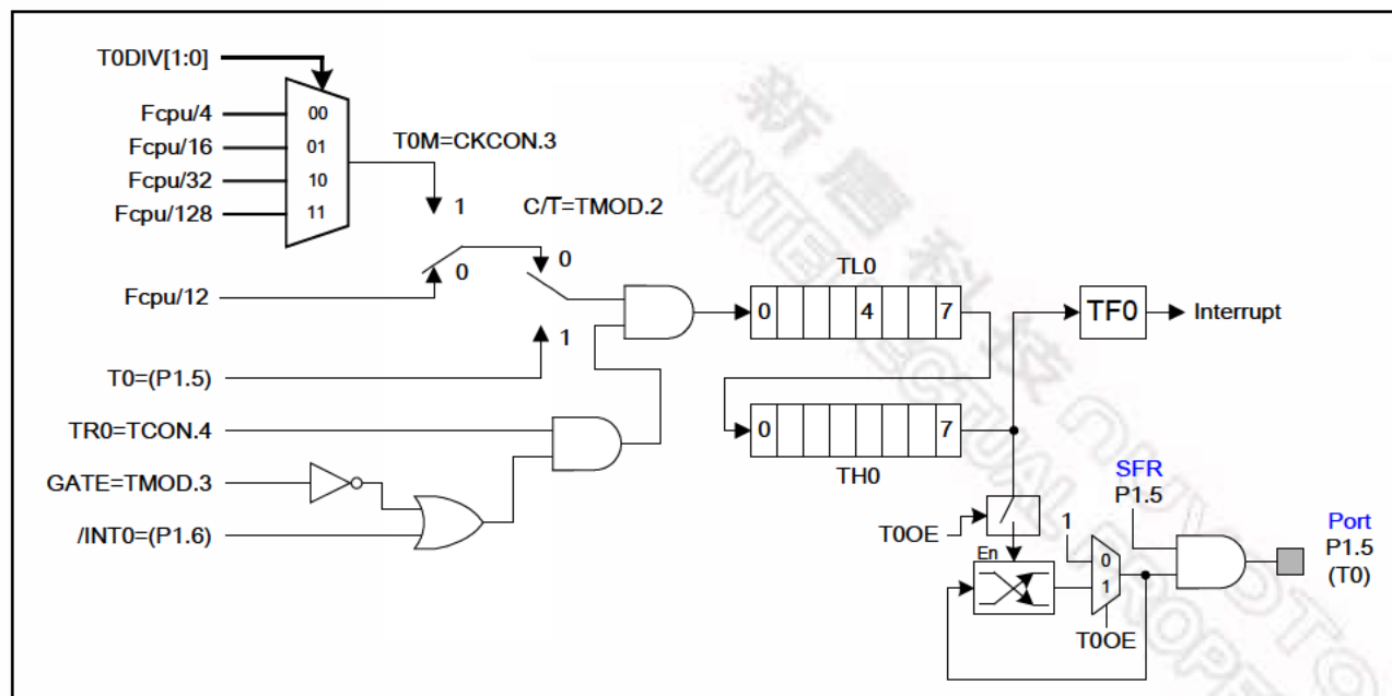
Figure 13-3 Timer 0 Mode 1
