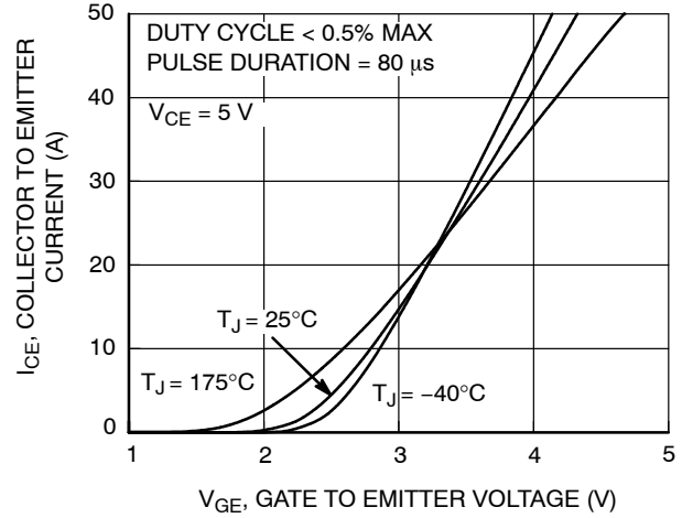
Figure 8. Transfer Characteristics
