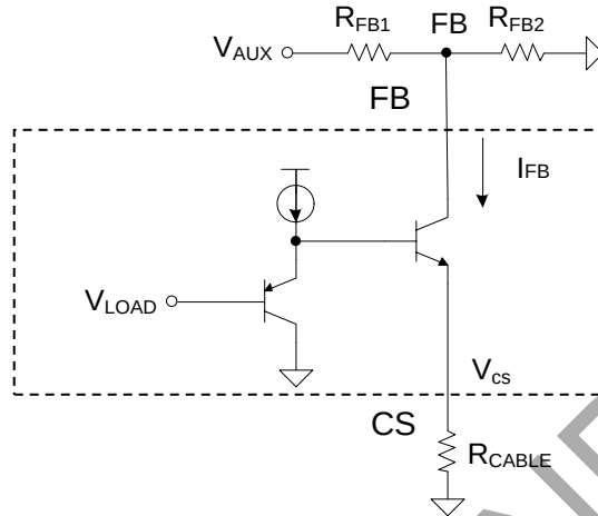
Figure 6. Cable Compensation
