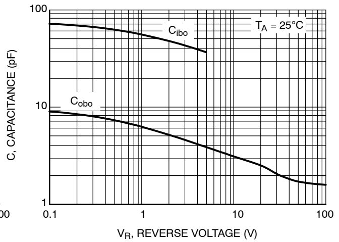
Figure 3. Capacitance
