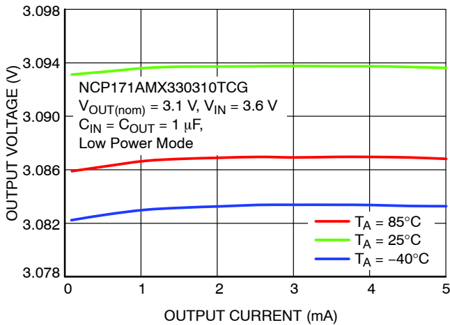
Figure 42. Output Voltage vs. Output Current in Low Power Mode
