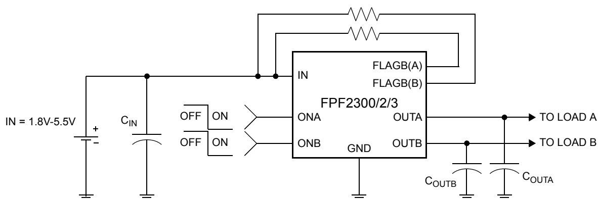
Figure 3. Typical Application
