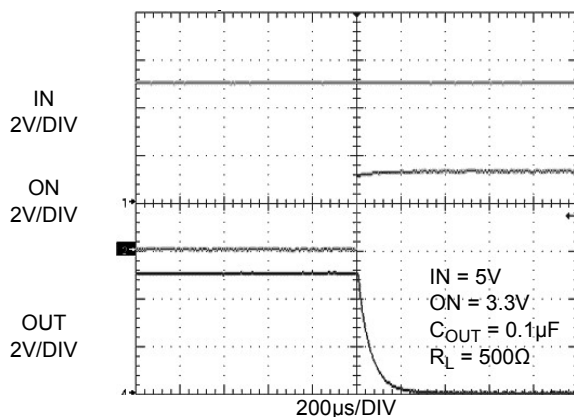
Figure 25. t_{OFF} Response
