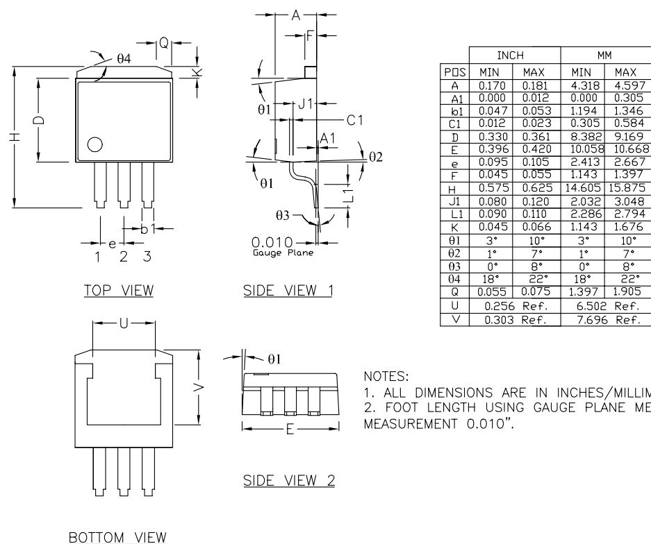
3-Pin TO-263 (U)
