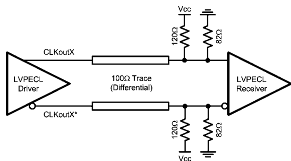
FIGURE 7. Differential LVPECL Operation, DC Coupling, Thevenin Equivalent
