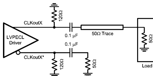
FIGURE 11. Single-Ended LVPECL Operation, AC Coupling
