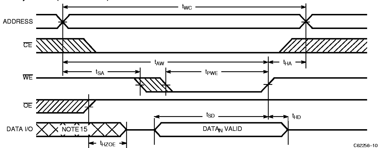
Write Cycle No. 1 (WE Controlled) [8,13,14]
