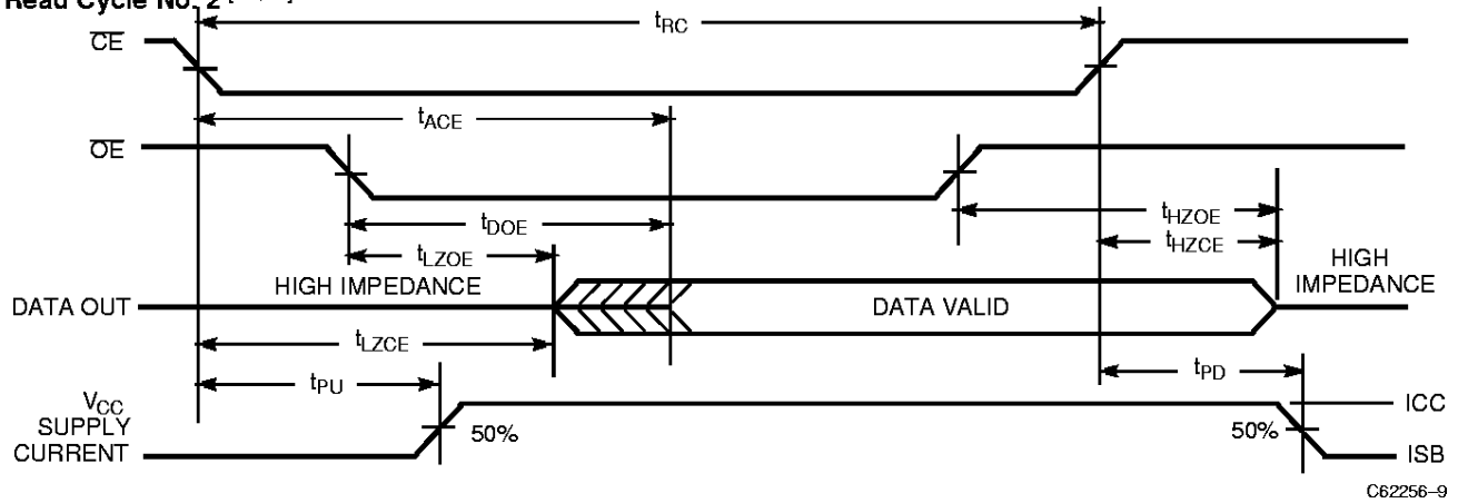
Read Cycle No. 2 [11,12]
