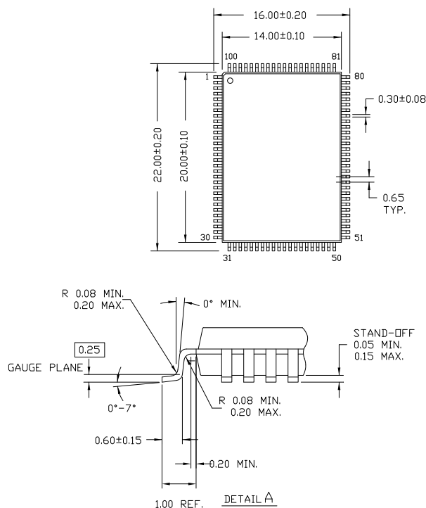
Figure 7. 100-Pin Thin Plastic Quad Flatpack (14 x 20 x 1.4 mm)
