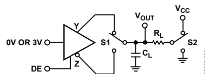
Figure 8. Driver Enable/Disable
