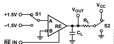
Figure 9. Receiver Enable/Disable
