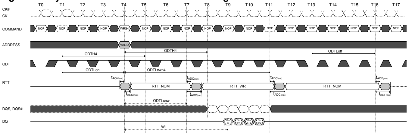
Figure 93. Dynamic ODT Behavior with ODT being asserted before and after the write
