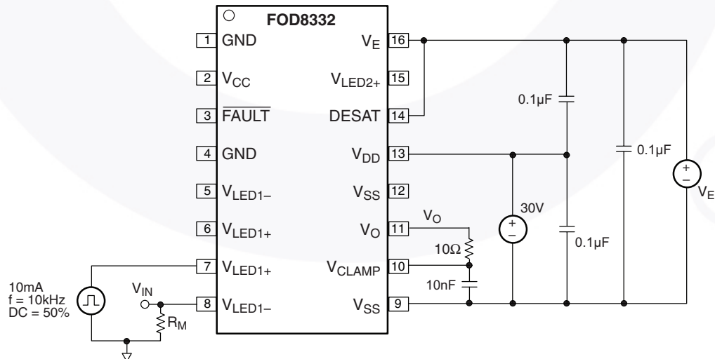
Figure 47. Propagation Delay ( t_{\text{PLH}} , t_{\text{PHL}} ), Rise Time ( t_R ), Fall Time ( t_F ), Pulse Width Distortion (PWD) Test Circuit
