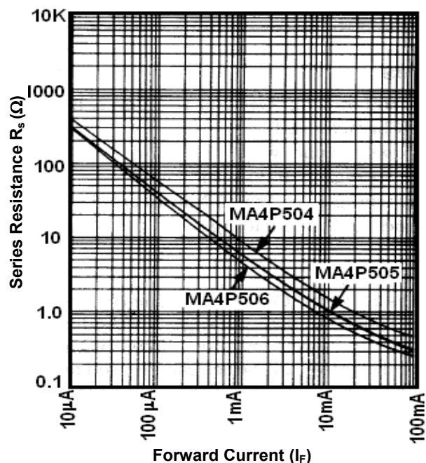
Forward Current vs. Series Resistance MA4P504, MA4P505 and MA4P506
