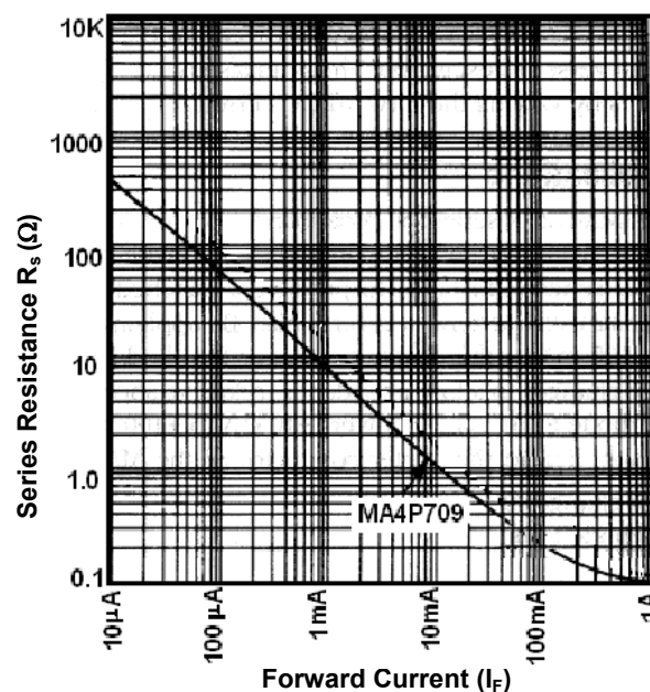
Forward Current vs. Series Resistance MA4P709
