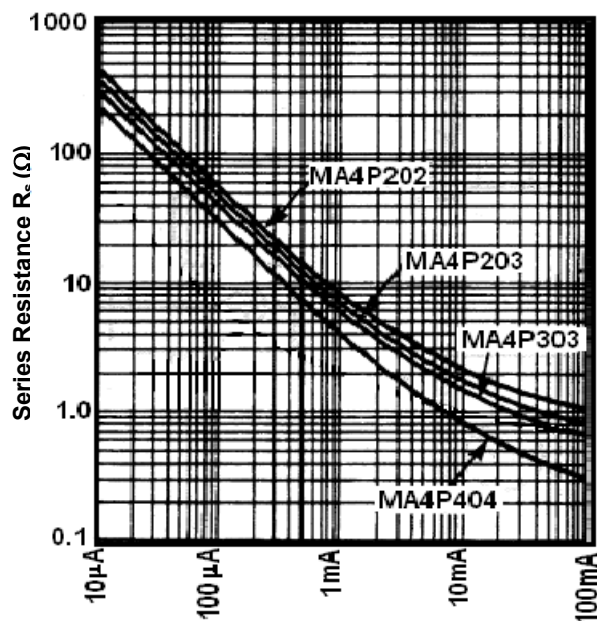
Forward Current vs. Series Resistance MA4P202, MA4P203, MA4P303 and MA4P404
