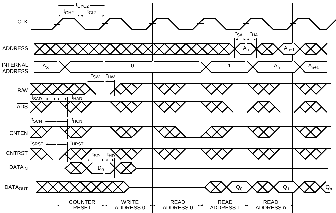
Figure 16. Counter Reset (Pipelined Outputs) [47, 48, 49, 50]
