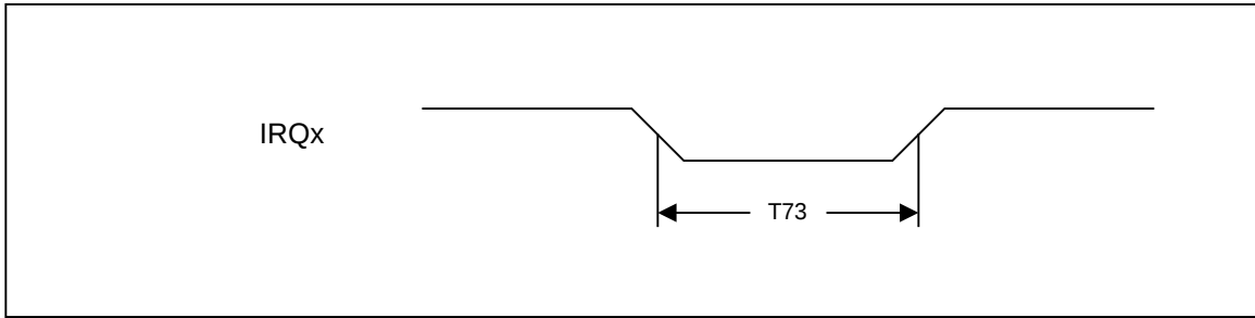
FIGURE 9 - INTERRUPT TIMING
