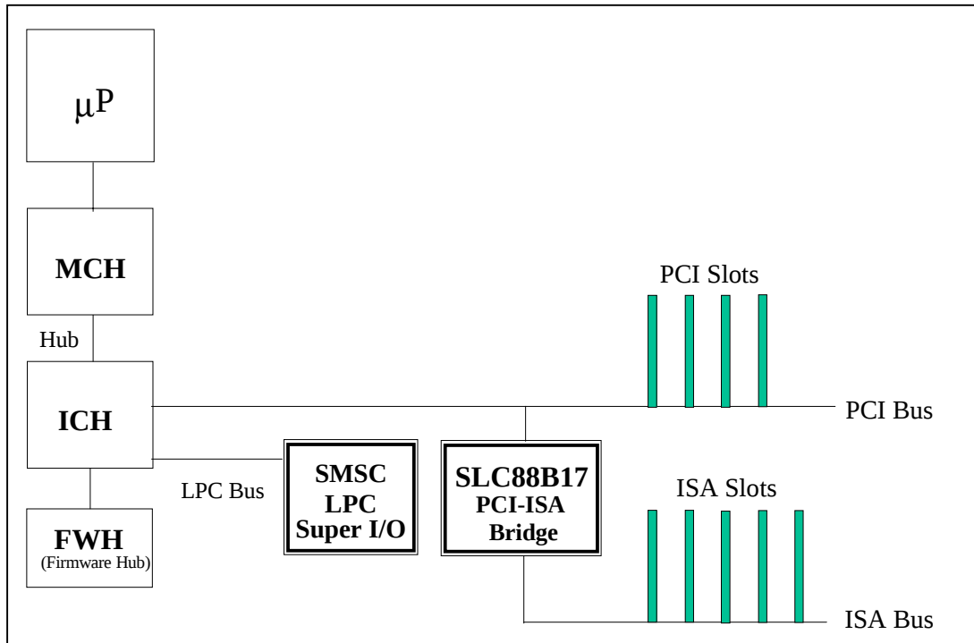
FIGURE 1 - DESKTOP APPLICATION
