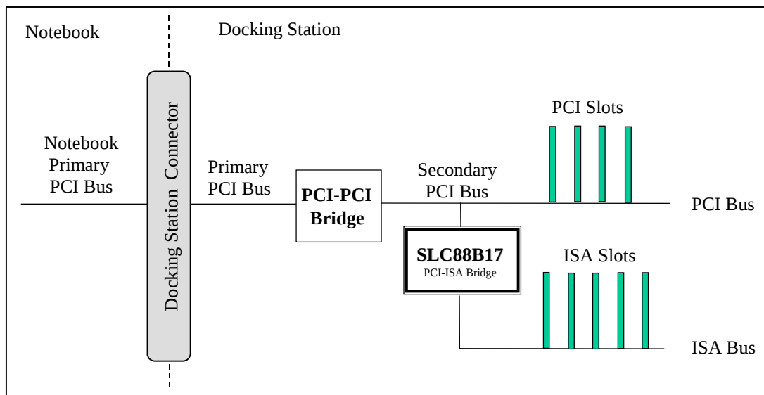
FIGURE 2 - NOTEBOOK DOCKING STATION APPLICATION
