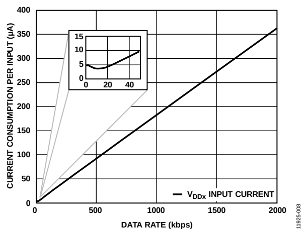
Figure 11. Current Consumption per Input vs. Data Rate for 3.3 V, EN_x = \text{Low Operation}
