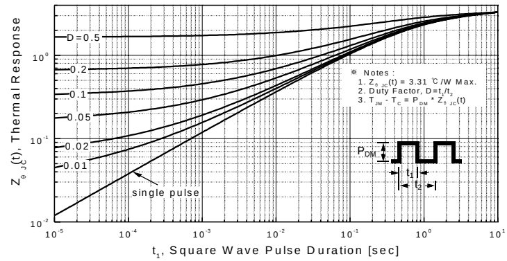
Figure 11-2. Transient Thermal Response Curve for IRFS730B
