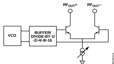
Figure 18. Output Stage
