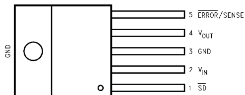
Top View TO220-5 Package Bent, Staggered Leads
