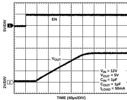
Figure 18. Start-Up Time
