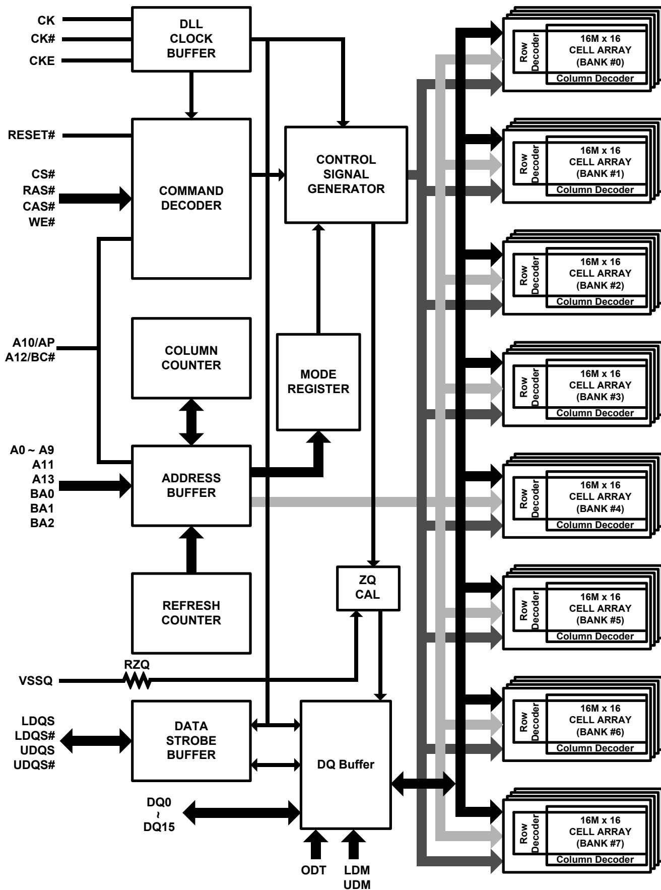
Figure 2. Block Diagram
