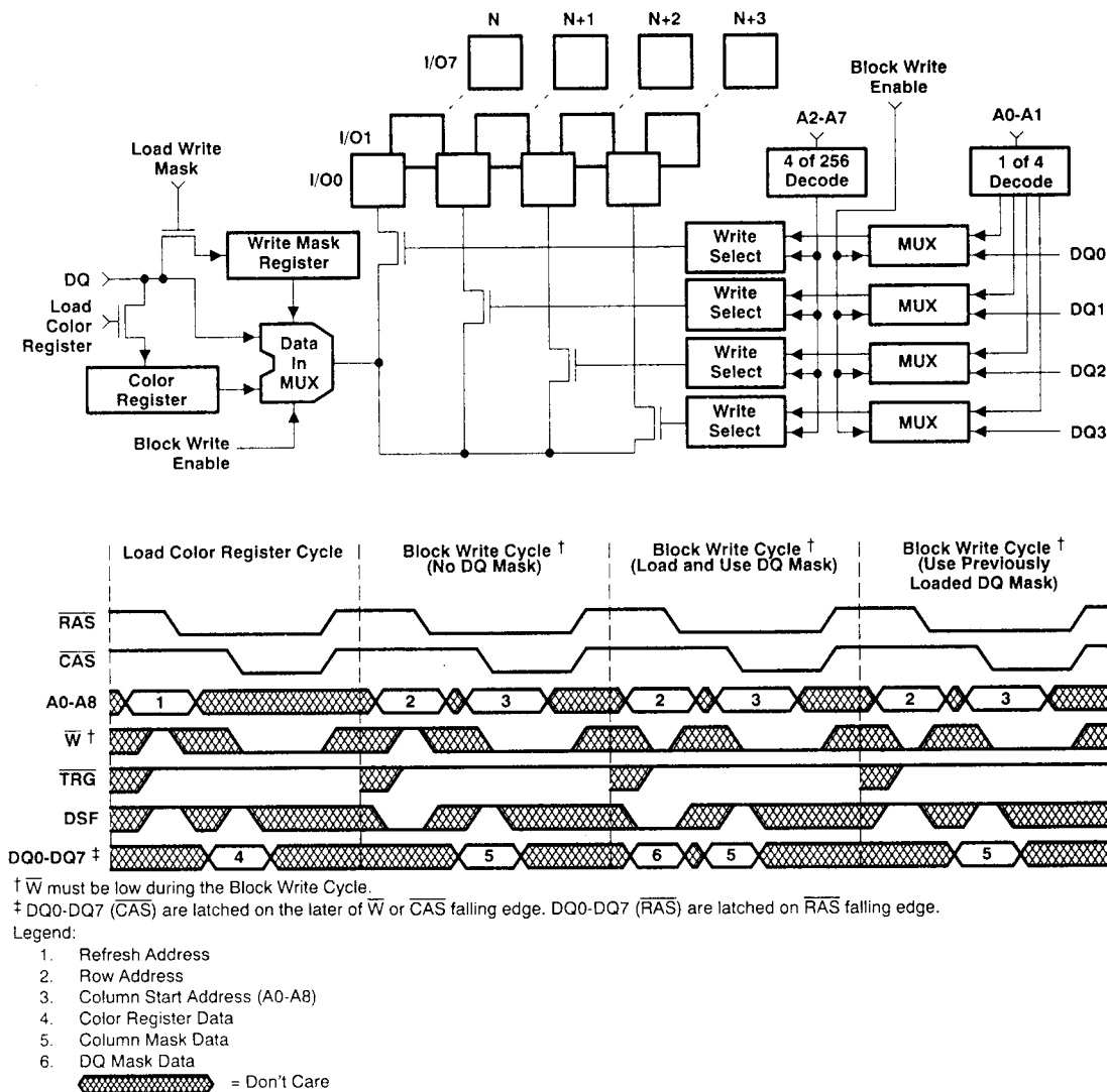
Figure 1. Block Write Diagram
