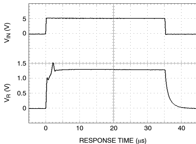
Figure 4. LM4041 – 1.225 V ( R_S = 30 k)
