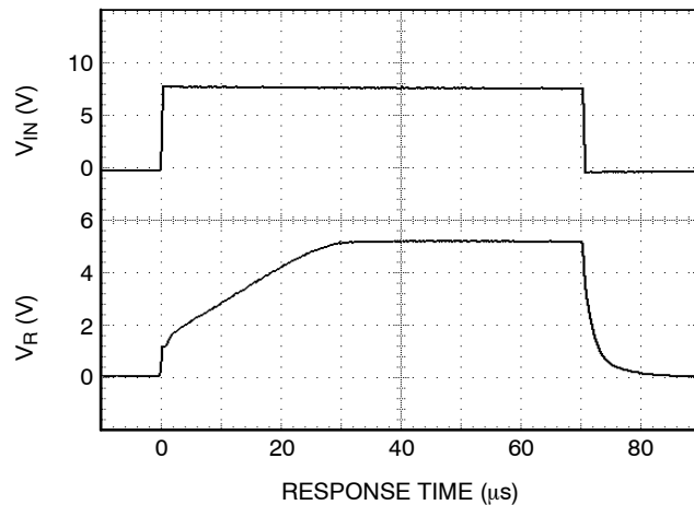
Figure 3. LM4040 – 5 V ( R_S = 30 k)
