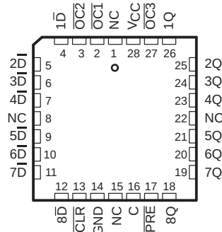
SN74ALS29846 . . . FN Package (Top View)
