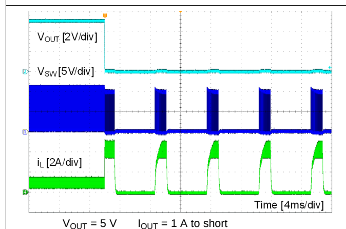
Figure 32. Short Protection
