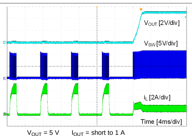
Figure 33. Short Recovery
