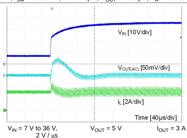
Figure 31. Line Transient
