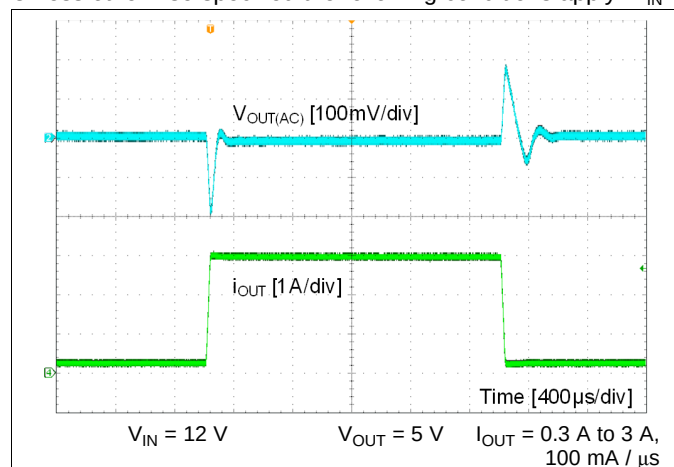
Figure 30. Load Transient
