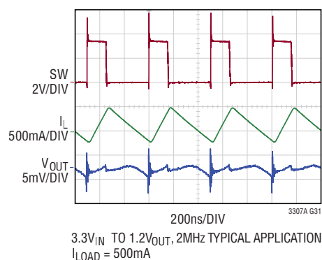
Switching Waveforms, Forced Continuous Mode
