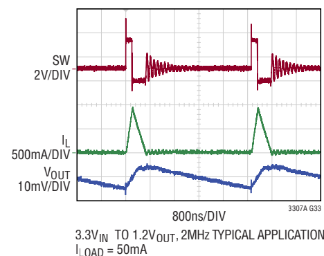
Switching Waveforms, Burst Mode Operation
