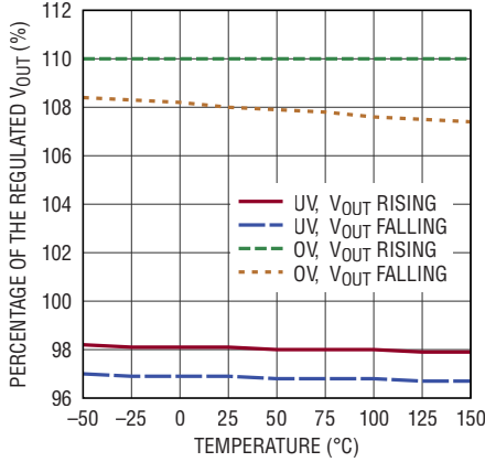
UV, OV PGGOOD Thresholds
