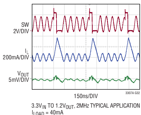
Switching Waveforms, Pulse-Skipping Mode
