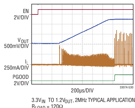
Start-Up Waveforms Burst Mode
