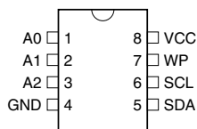
8-lead TSSOP
