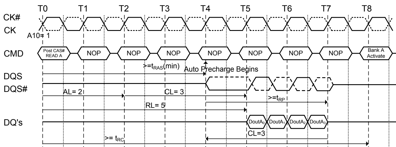
Figure 39. Burst read operation with auto precharge followed by activation to the same bank ( t_{RC} Limit): RL=5(AL=2, CL=3, \text{internal } t_{RCD}=3, BL=4, t_{RTP} \leq 2 \text{ clocks})
