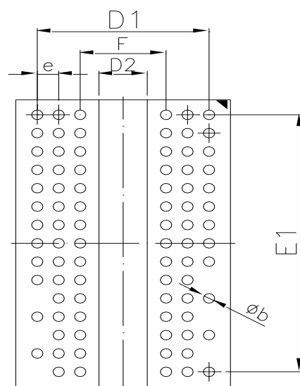
Bottom View
