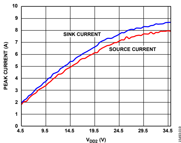
Figure 19. Peak Current vs. V_{DD2} , 2 \Omega Resistor
