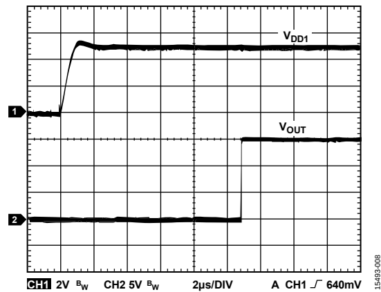
Figure 8. Typical V_{DD1} Delay to Output Waveform, V_{IN} = V_{DD1}
