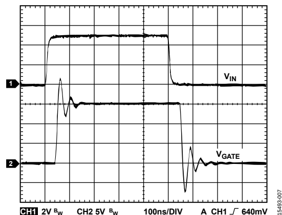
Figure 7. ADuM4120-1 V_{IN} to V_{GATE} Waveform for 2 nF Load, 0 \Omega Series Gate Resistor, V_{DD2} = 15 V
