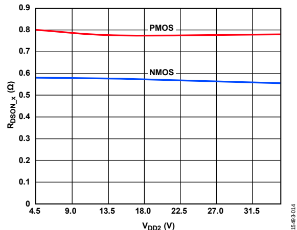
Figure 14. R_{DS(on)_x} vs. V_{DD2}
