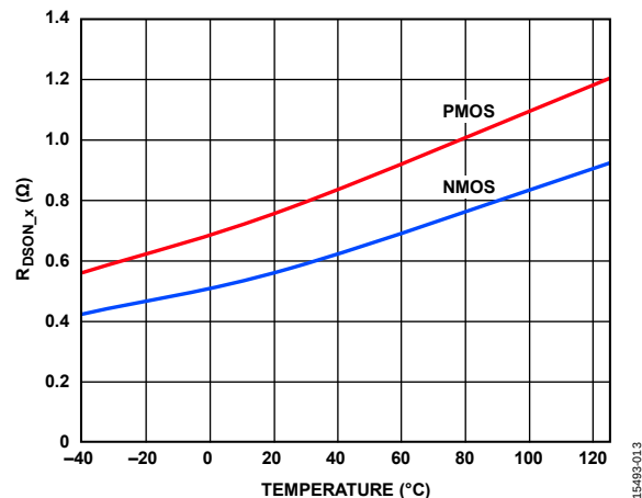
Figure 13. R_{DS(on)_x} vs. Temperature
