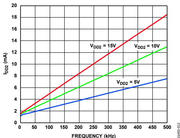
Figure 12. I_{DD2} vs. Switching Frequency, 2\text{ nF} Load
