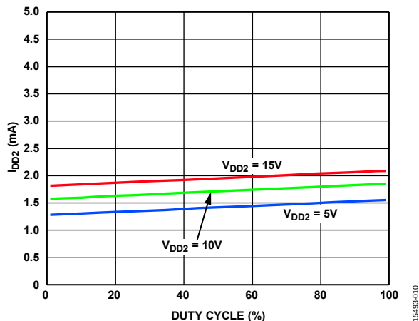
Figure 10. I_{DD2} vs. Duty Cycle, V_{DD1} = 5\text{ V} , f_{SW} = 10\text{ kHz} , 2\text{ nF} Load
