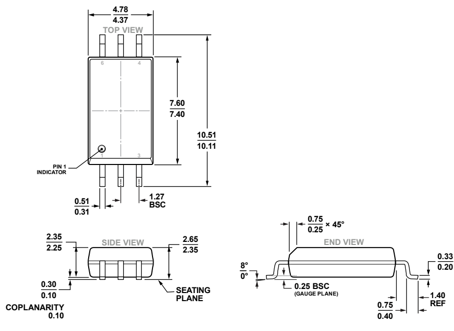
Figure 27. 6-Lead Standard Small Outline Package, with Increased Creepage [SOIC_IC] Wide Body (RI-6-1)
