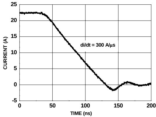
Figure 13. FDMC0202S SyncFET body diode reverse recovery characteristic
