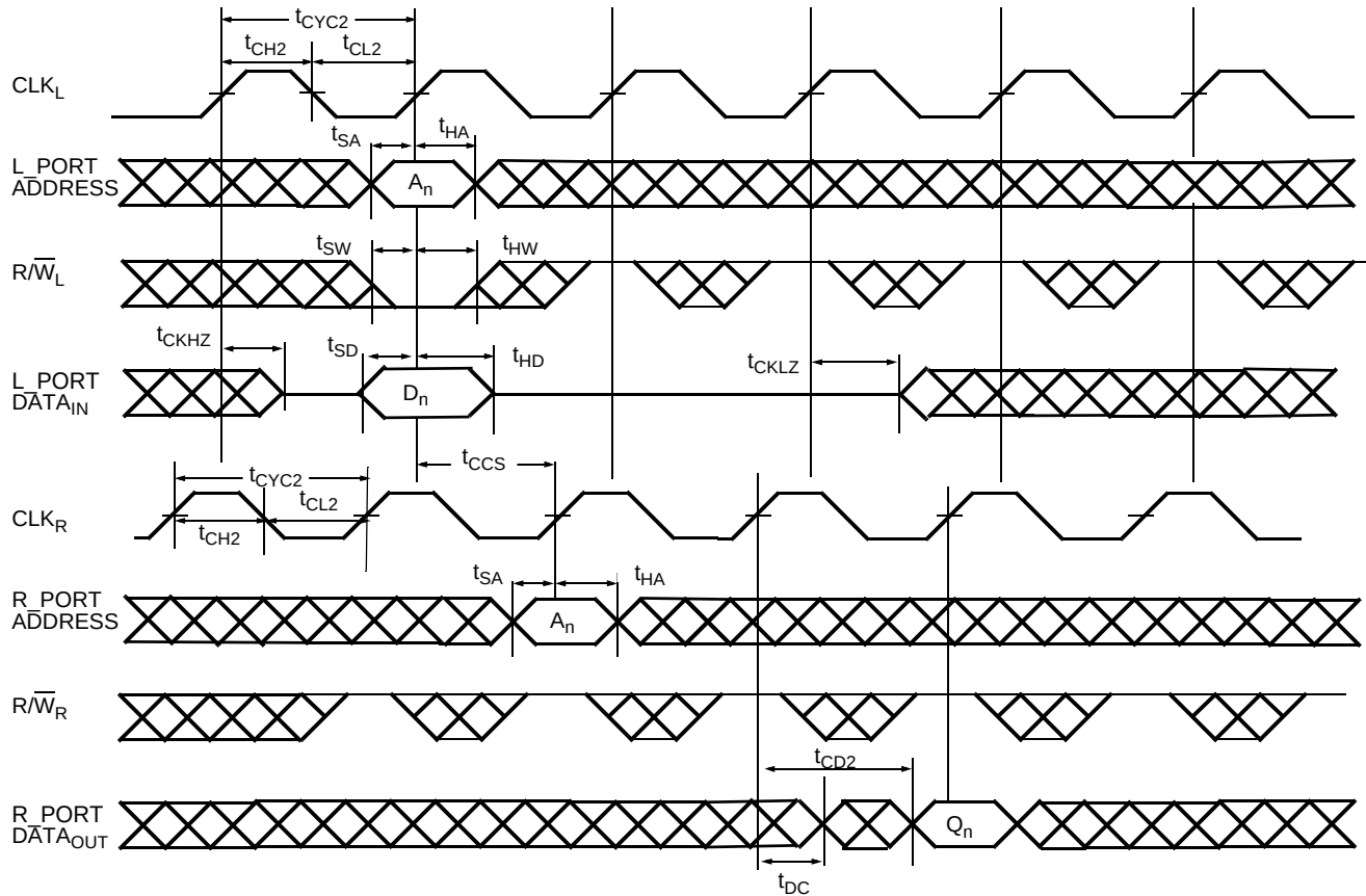
Figure 21. Left_Port (L_Port) Write to Right_Port (R_Port) Read [55, 56, 57]
