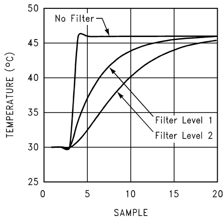
a) Step Response
