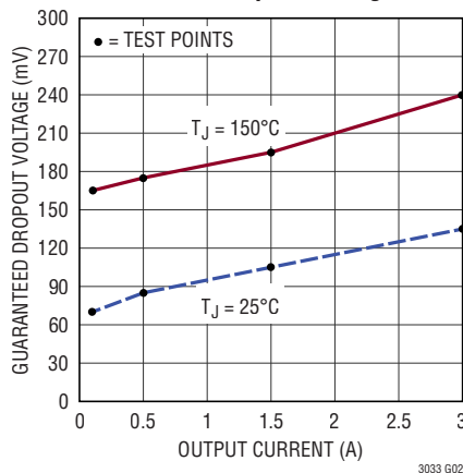
Guaranteed Dropout Voltage
