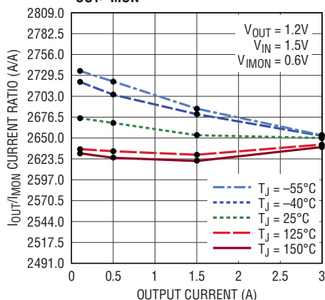
I OUT /I MON Current Ratio
