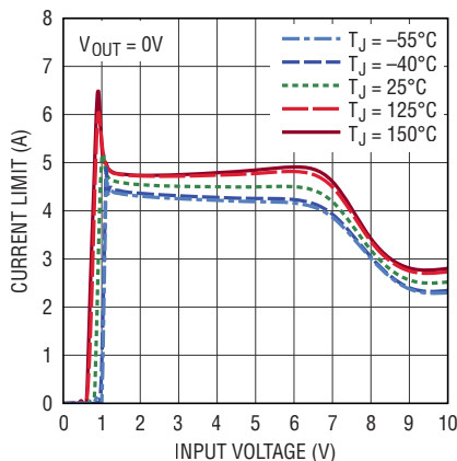
Internal Current Limit
