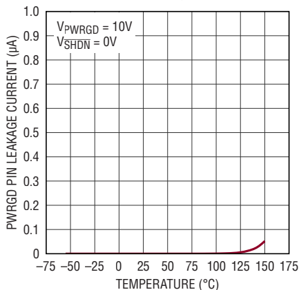
PWRGD Pin Leakage Current
