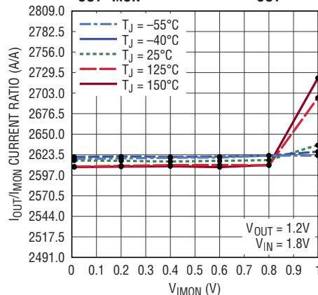
I OUT /I MON Current Ratio, I OUT = 3A
