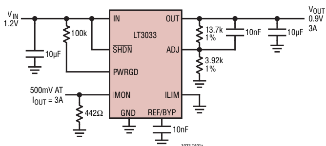
1.2V to 0.9V, 3A VLDO Regulator
