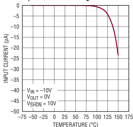
Input Reverse Leakage Current
