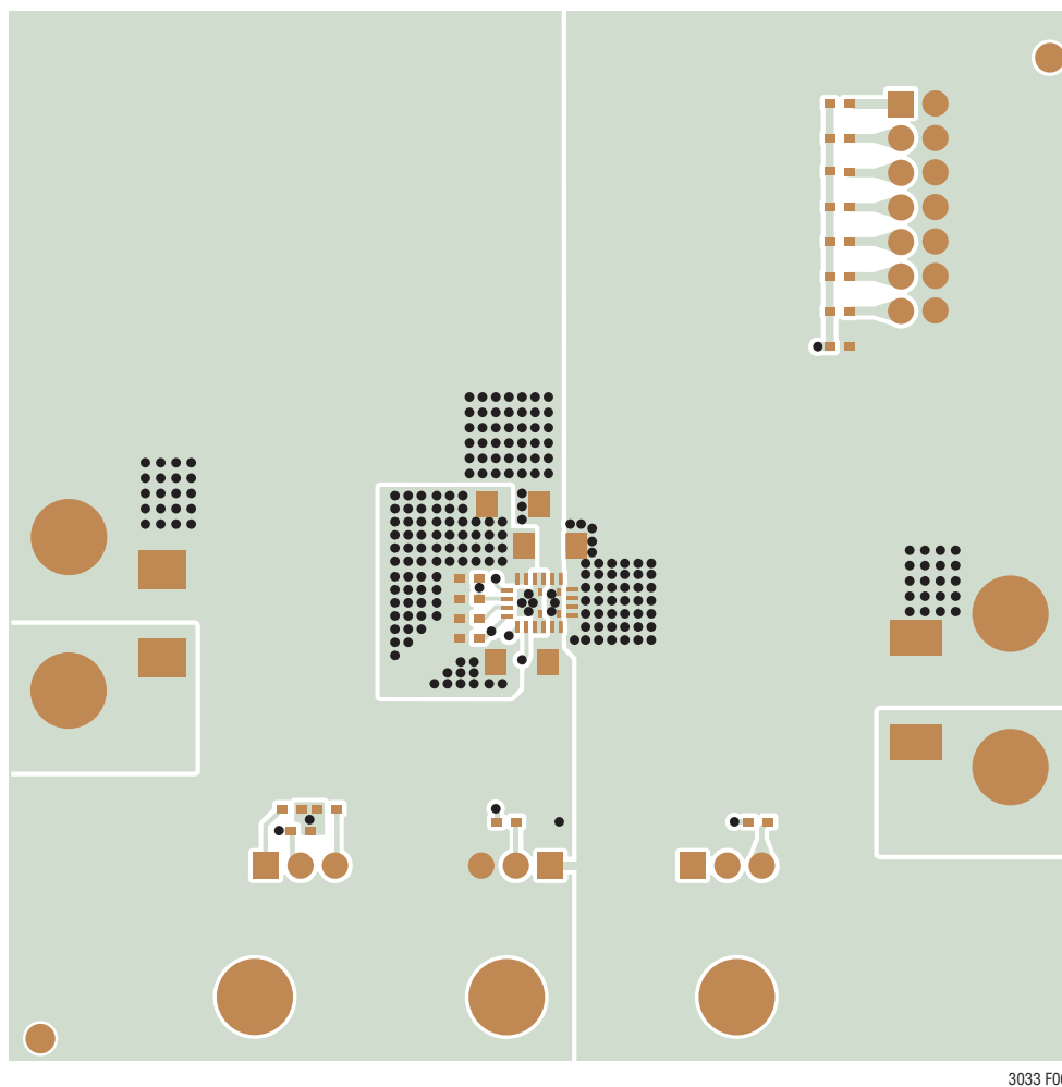
Figure 6. Recommended Layout (Demo Board DC2362A)
