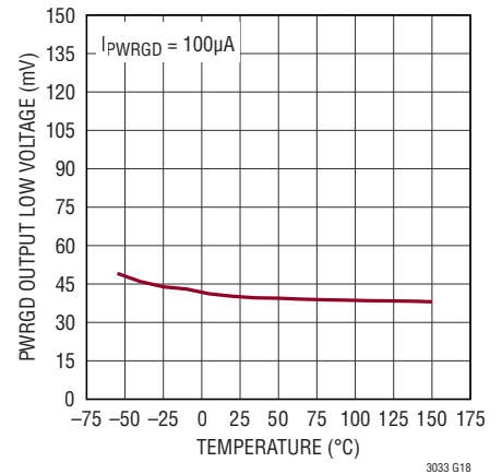
PWRGD Output Low Voltage
